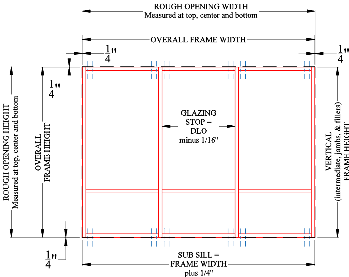
FIGURE 1.0 MOCK UP
