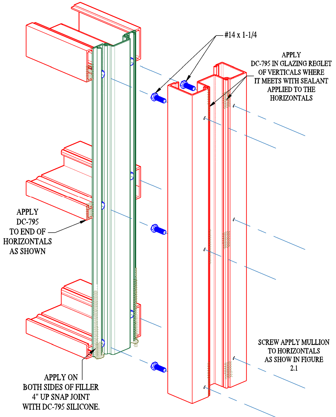
FIGURE 2.2 MULLION INSTALLATION
