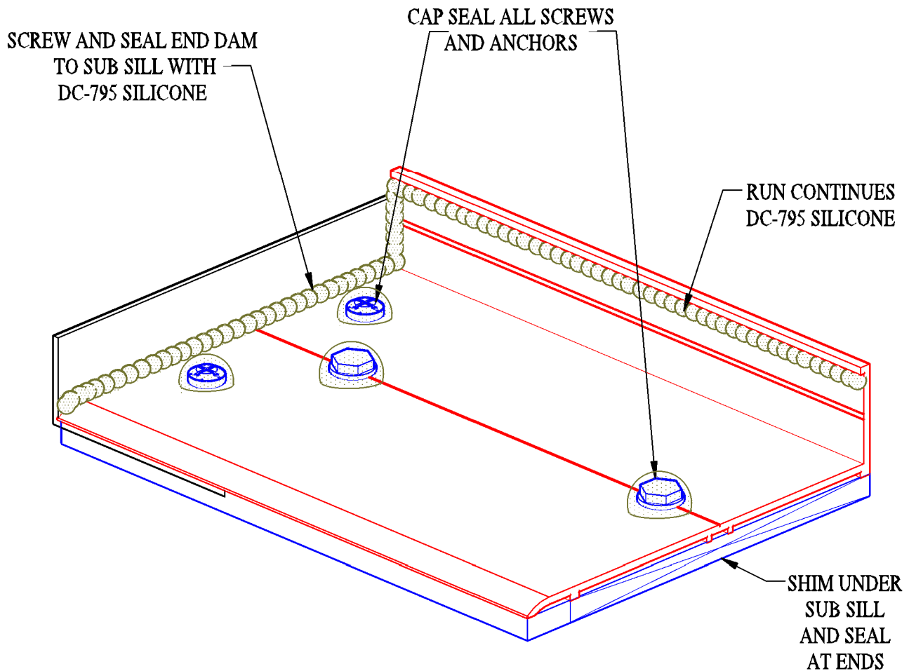
FIGURE 2.0 SILL FLASHING INSTALLATION
