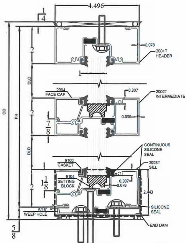
Horizontal Detail
